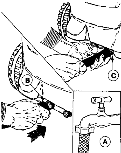
Water circuit connection.
